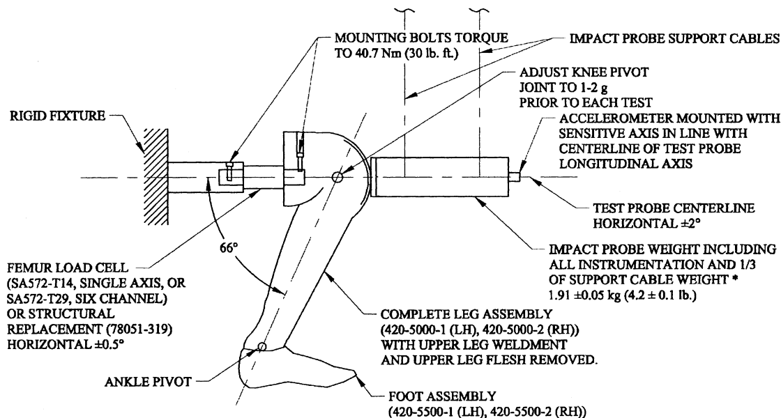
FIGURE T6 KNEE IMPACT TEST SETUP SPECIFICATIONS
