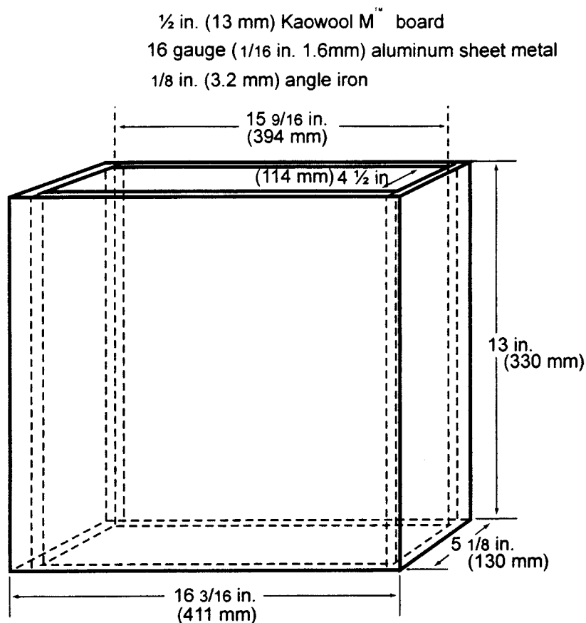
Figure 2 - Internal Chimney
