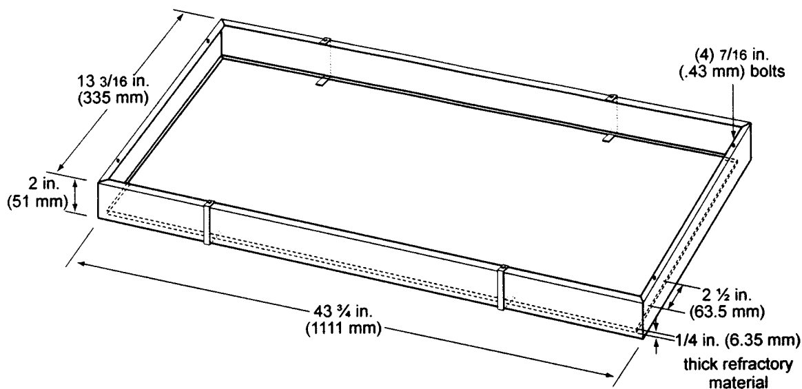
Figure 4 - Sliding Platform
