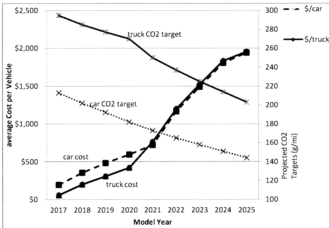
Figure 7. Year on Year Progression of Projected (Target) CO 2 Standards and Average Cost Per Vehicle
