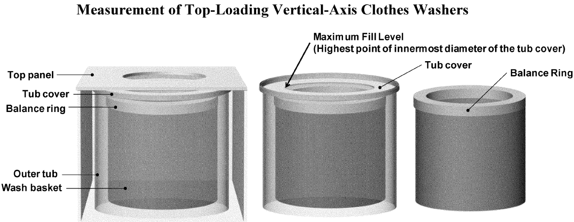
Figure 3.1.4.1—Maximum Fill Level for the Clothes Container Capacity
