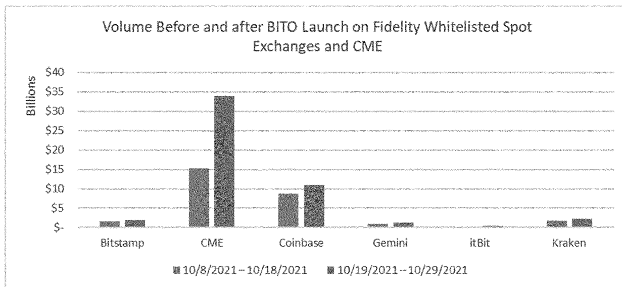
Figure 12: Volume Comparison Before and After BITO Launch on Fidelity Whitelisted Spot Exchanges and CME
