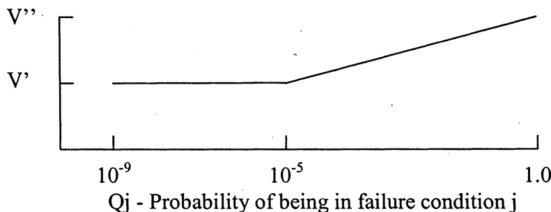
Figure 3 Clearance Speed
