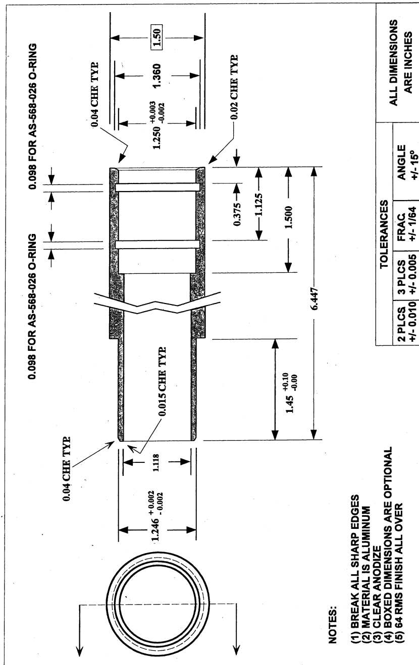
FIGURE O-1.DOWNTUBEEXTENSION
