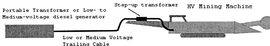
Figure 2 - Power source - 75.829(c) (2) 480 or 995 volts to a step-up transformer to 2300 volts for tramping
