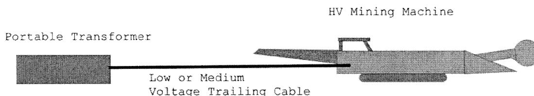
Figure 1-Power Source-75.829(c) (1) 995 volts used for tramping
