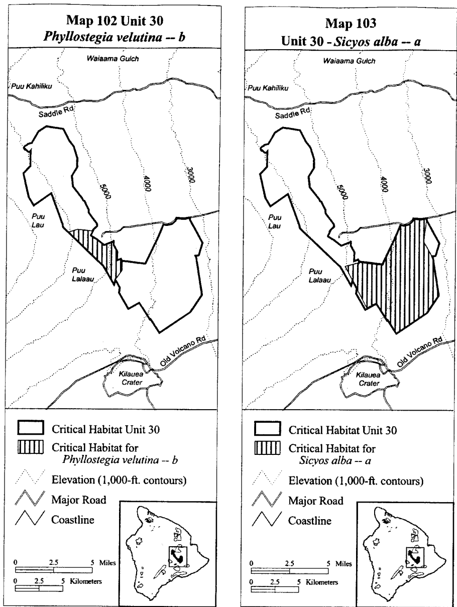
(103) Hawaii 30— Sicyos alba —a (6,266 ha, 15,483 ac)
