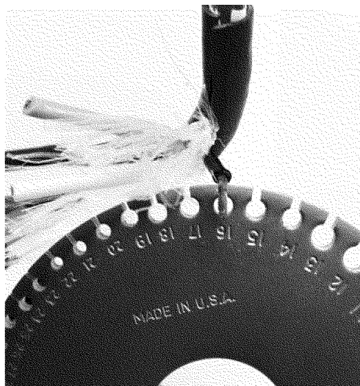
Picture 2: Measuring Wire Size
