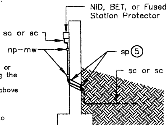
SKETCH C: Buried Service - Below Grade Entrance
