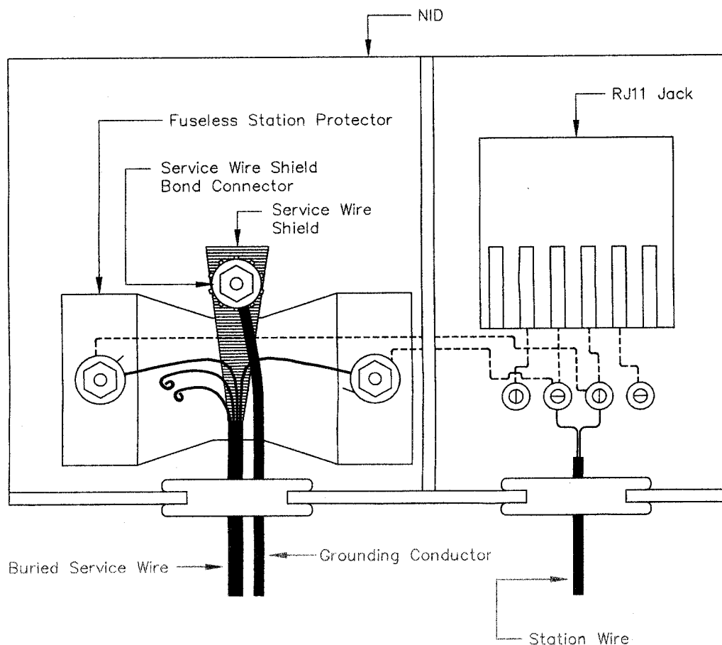
FIGURE 19 NID TERMINATIONS
