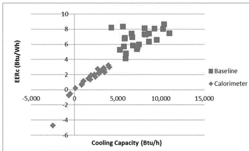
Figure III.1 Baseline and Calorimeter Results
