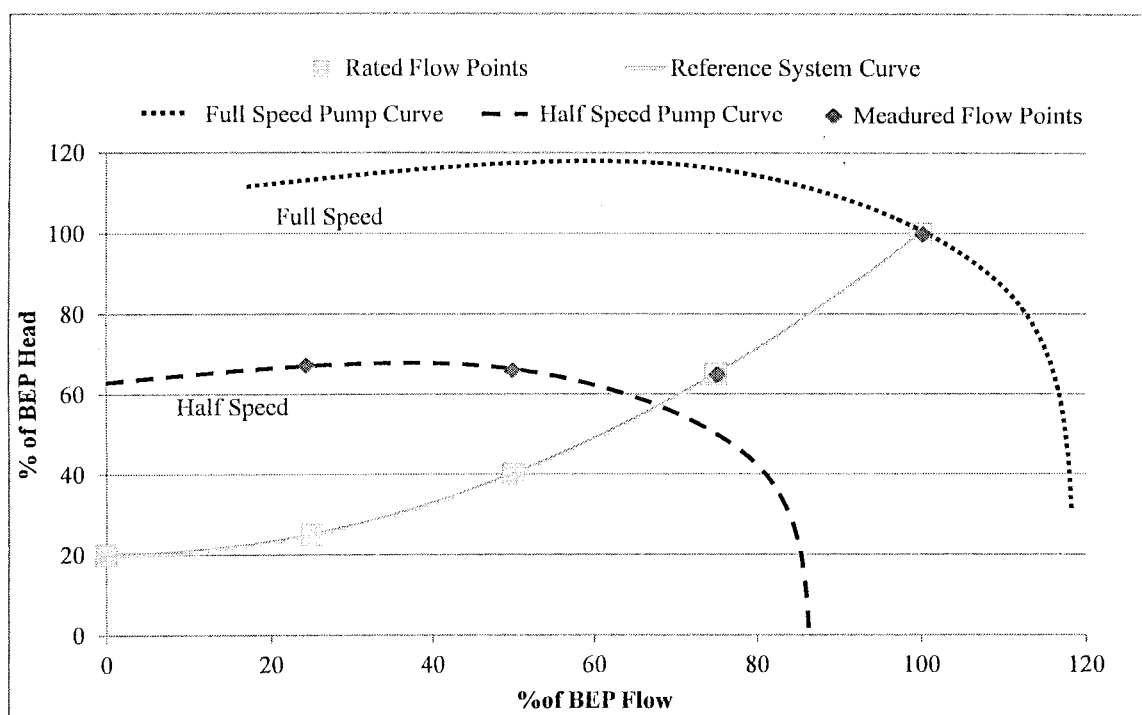
Figure III.3. Test Points Compared to Reference System Curve and Full Speed Pump Curve for a Theoretical Two-Speed Motor.
