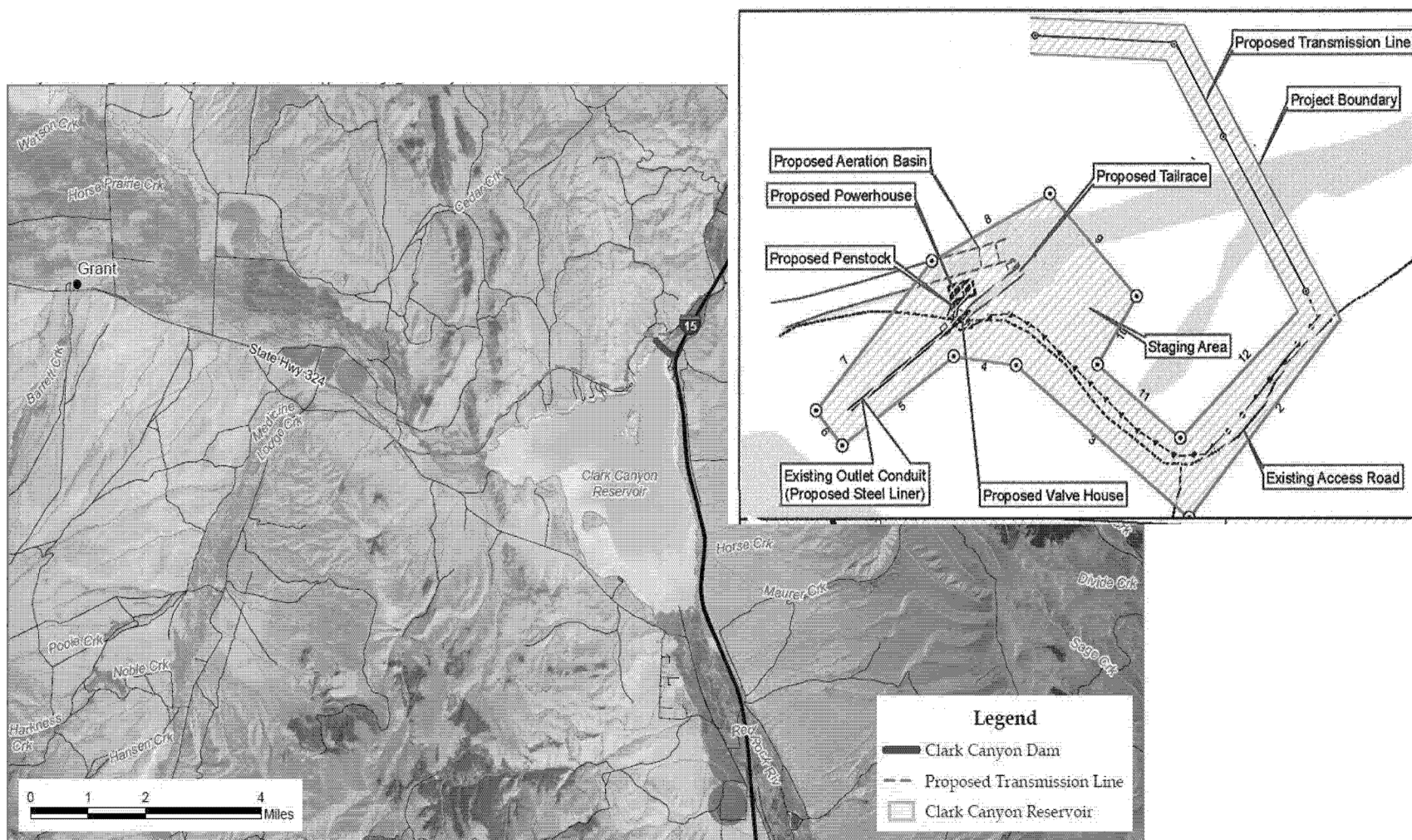
Figure 2. Clark Canyon Dam Project features (Source: Clark Canyon Hydro, LLC, 2015, as modified by staff).
