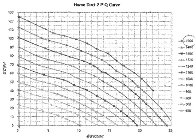
Figure 1: Blower Curves
